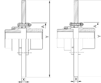
Brake Disc Type
